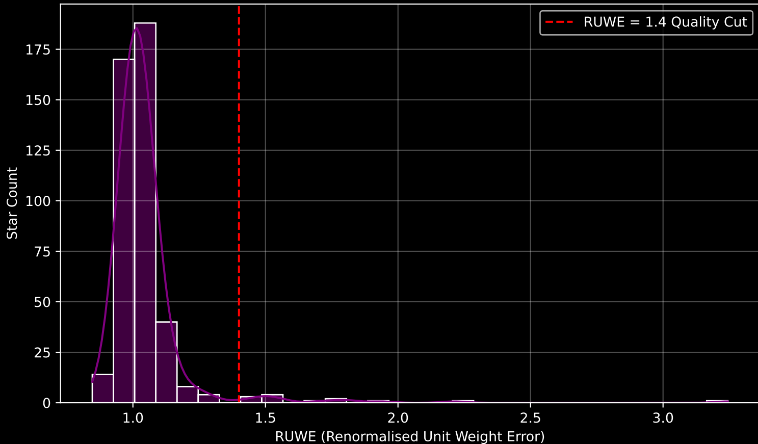
GAPOGEE DR17 Field [100-06] RUWE Distribution (n= 437)
