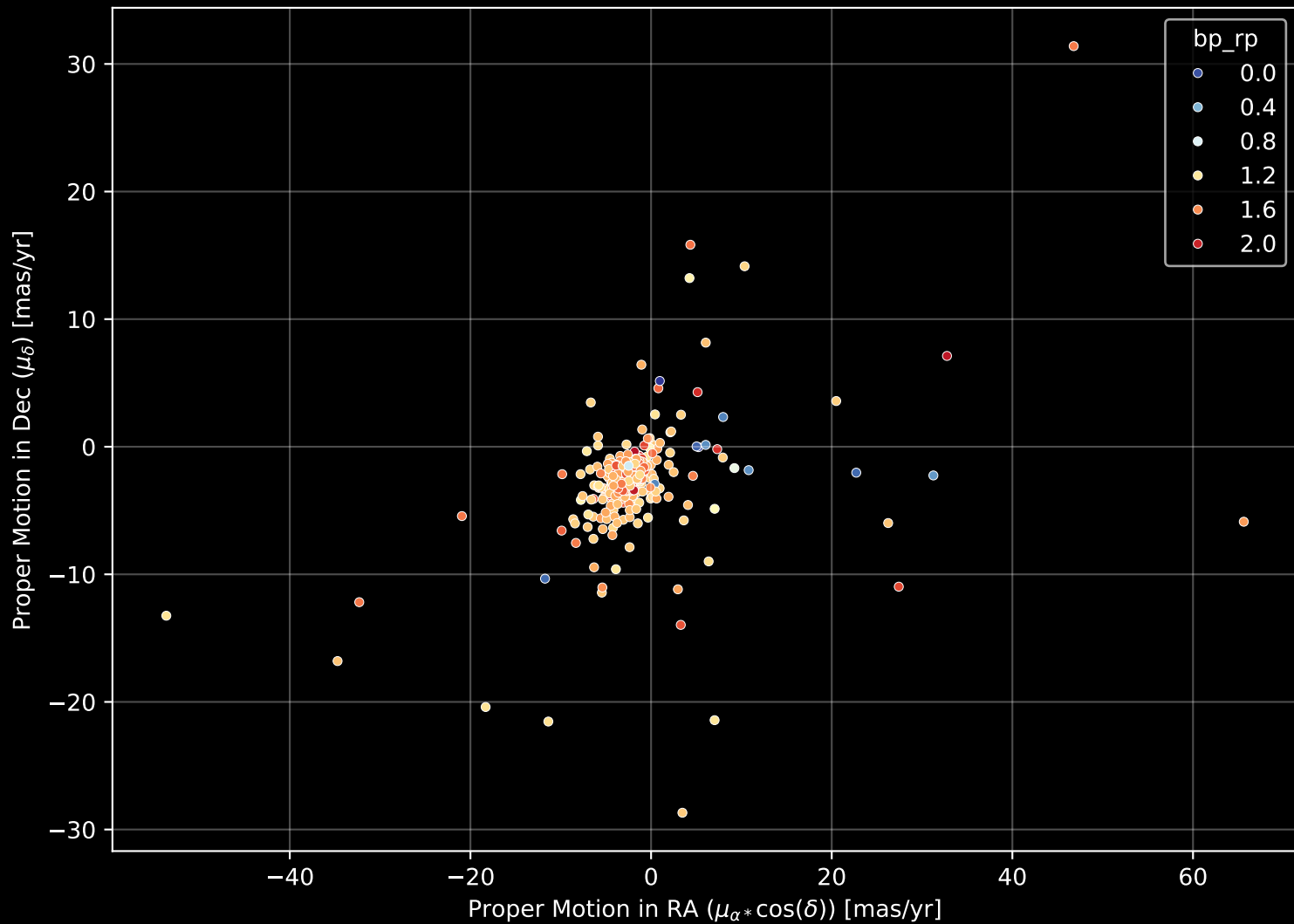
APOGEE DR17 Field: [100-06] Proper Motion Diagram (n= 444)
