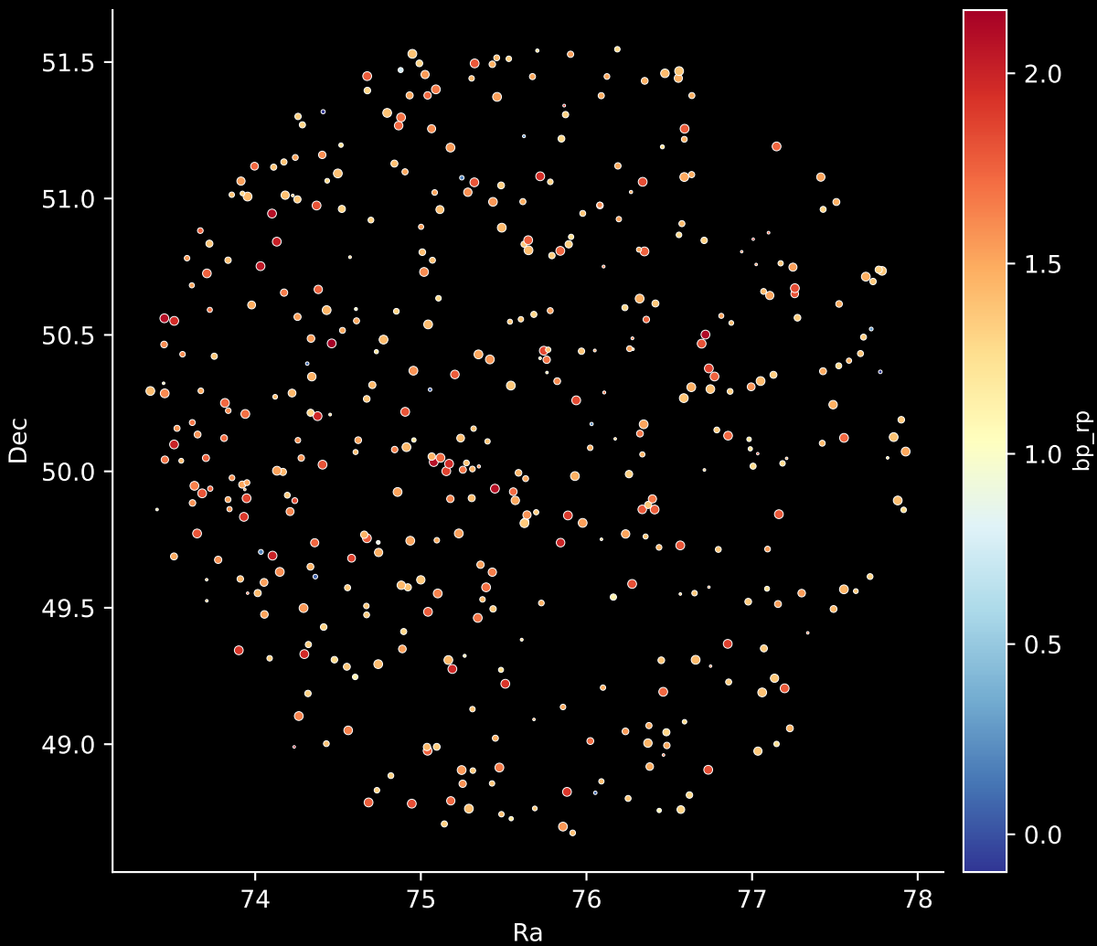
APOGEE DR17 Field: [100-06] Stars: 444
