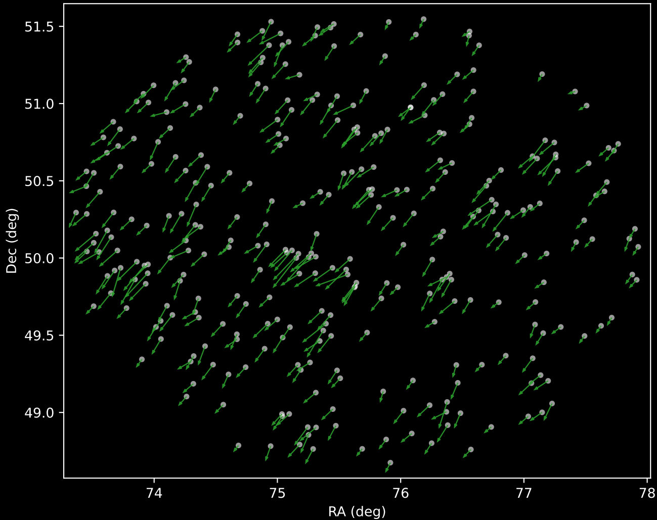
APOGEE DR17 Cluster 4 Proper Motion Vectors (n=319)
