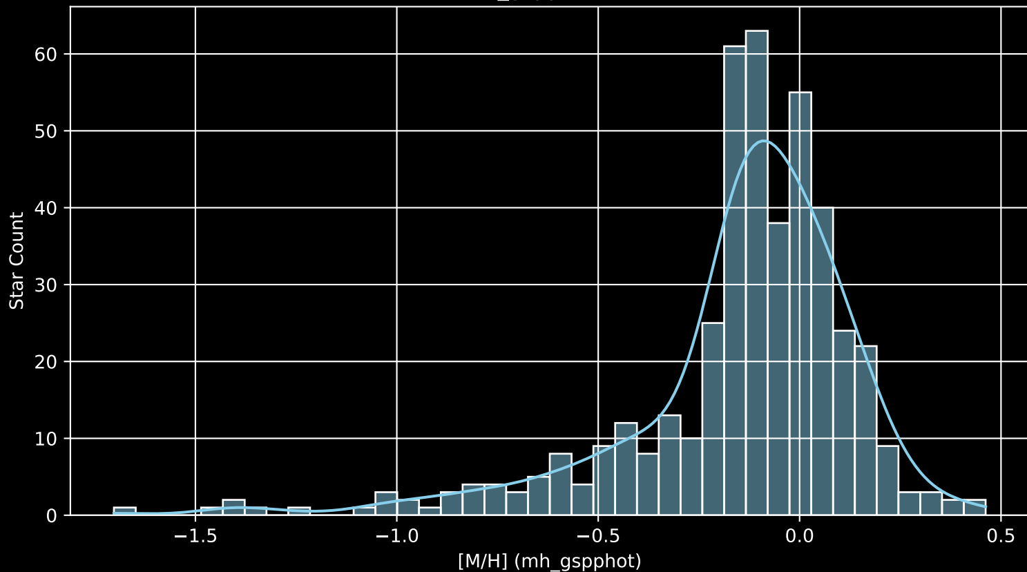
APOGEE DR17 Field: [100-06 [M/H] (mh_gspphot) (n= 443)
