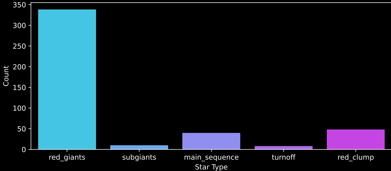
APOGEE DR17 Field: [100-06] Count plot of Star Type
