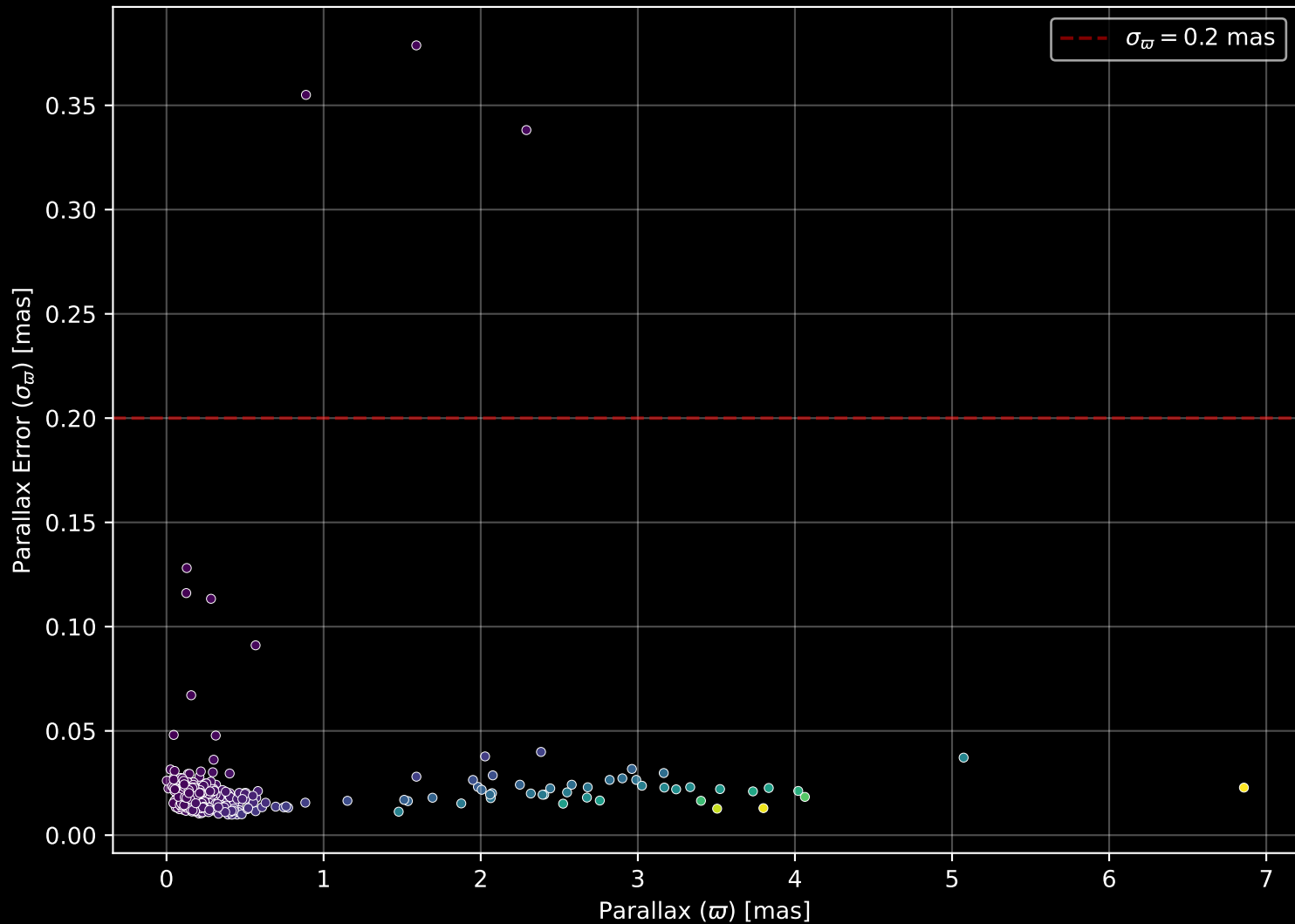
APOGEE DR17 Field: [100-06] Parallax Quality (n= 444)
